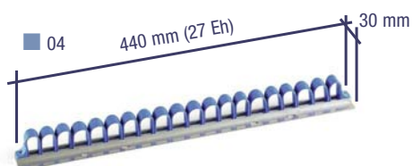
Supporti multiuso ART. F HD 7271 00 04 Dimensioni mm 440x30x35 h
