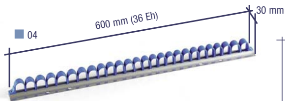
Supporti multiuso ART. F HD 7571 00 04 Dimensioni mm 600x30x35 h
